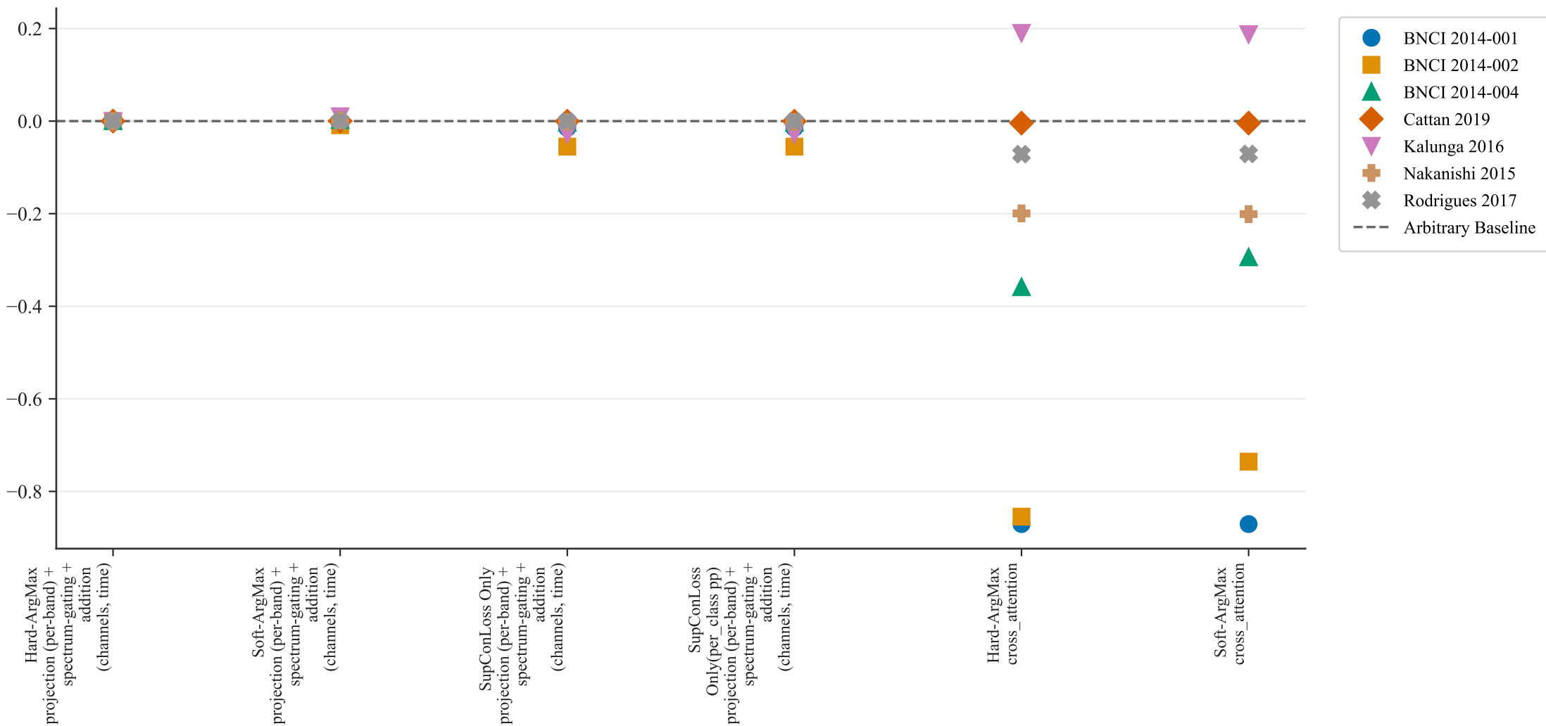
Paired Deltas by Config – Relative Delta
